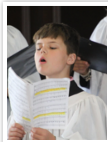
Children's Choir
